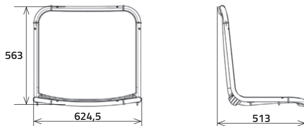
Jumbo without handle weight. 9,5 kg with handle 9,8 kg.
