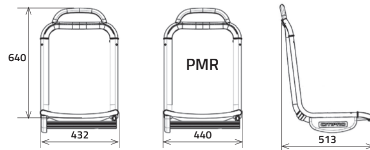
Basic without handle 4,9 kg with handle 5,5 kg. Pmr without handle 6,0 kg with handle 6,6 kg.
