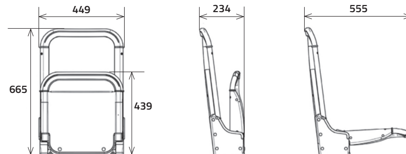
Tip up weight 8,8 kg
