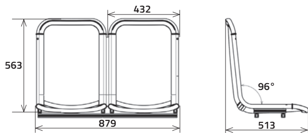
Basic double without handle weight. 9,8 kg with handle 10,3 kg.
