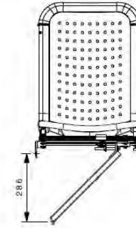
Cantilever frame
