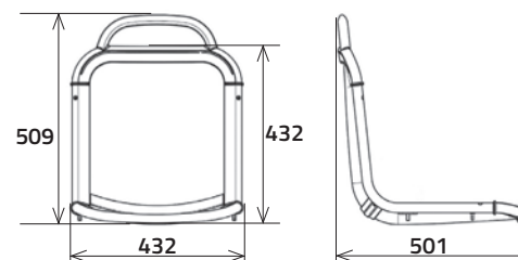
Junior without handle 4,2 kg with handle 4,8 kg.
